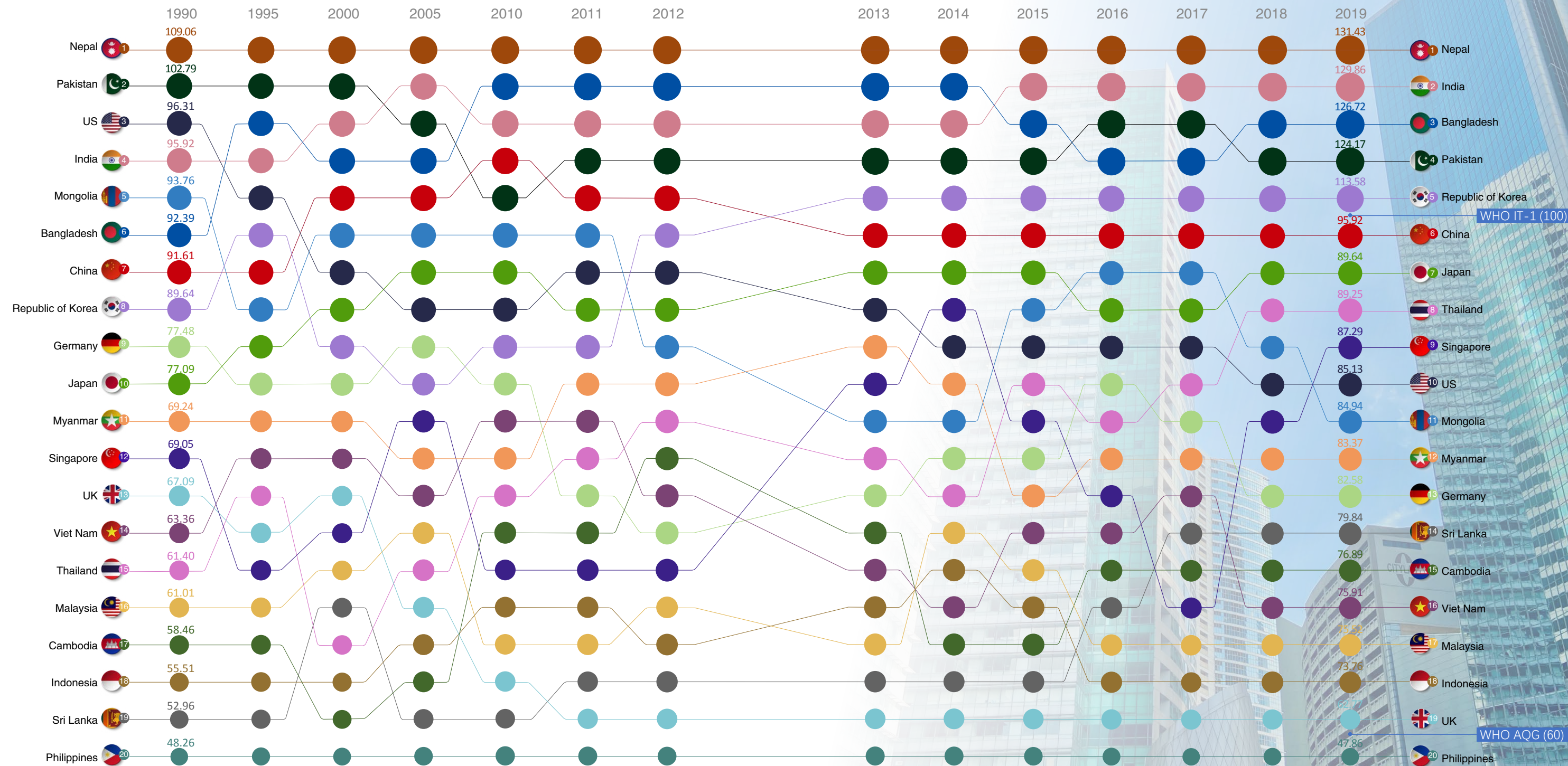
Figure 1.5 O 3 Exposure Concentration in Ozone Season and Ranking by Country, 1990-2019 Note: Ozone season is the six consecutive months with the highest O 3 concentration levels in a year. The figure shows population-weighted annual average O 3 concentrations (µg/m 3 ).
