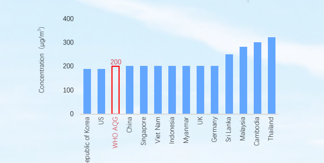
Figure 1.13 NO 2 1-hour Average Concentration Limits of Various Countries
