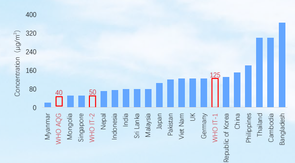
Figure 1.10 SO 2 24-hour Average Concentration Limits of Various Countries
