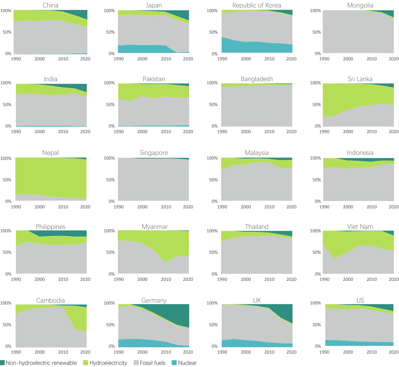
Figure 4.7 Changes in Installed Power Generation Capacity Structure, 1990-2019
