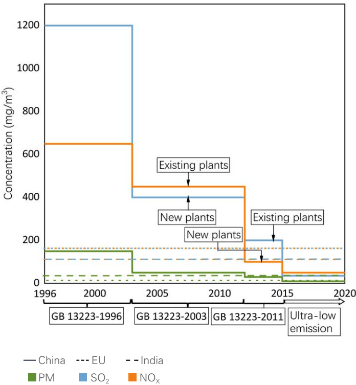
Figure 4.9 Course of Upgrades for the Power Sector's Emission Standards in China
