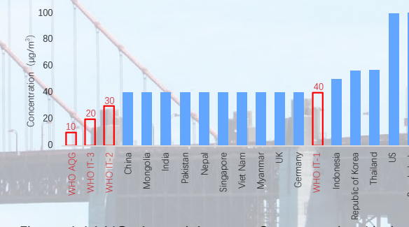
Figure 1.14 NO 2 Annual Average Concentration Limits of Various Countries
