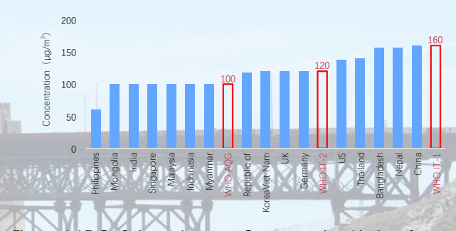
Figure 1.15 O 3 8-hour Average Concentration Limits of Various Countries
