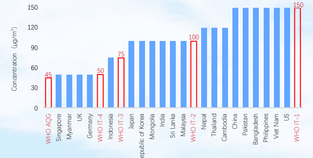
Figure 1.11 PM 10 24-hour Average Concentration Limits of Various Countries
